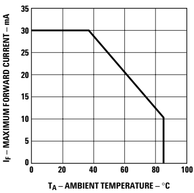
Figure 7. Maximum forward current vs. ambient temperature.
